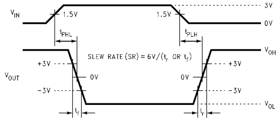
FIGURE 2. Driver Propagation Delay and Slew Rate Timing
