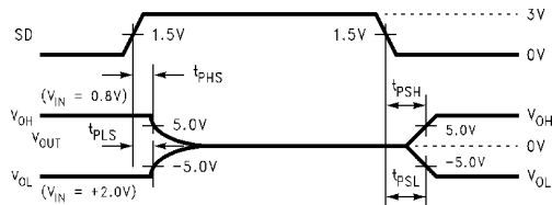
FIGURE 6. Driver SHUTDOWN (SD) Delay Timing
