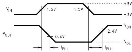
FIGURE 4. Receiver Propagation Delay Timing
