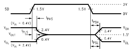
FIGURE 8. Receiver SHUTDOWN (SD) Delay Timing
